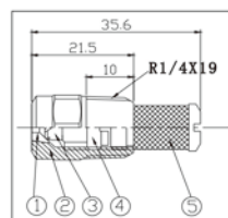
1.Orifice 2.Body 3.Cyclone Core 4.Plug 5.strainer mesh
